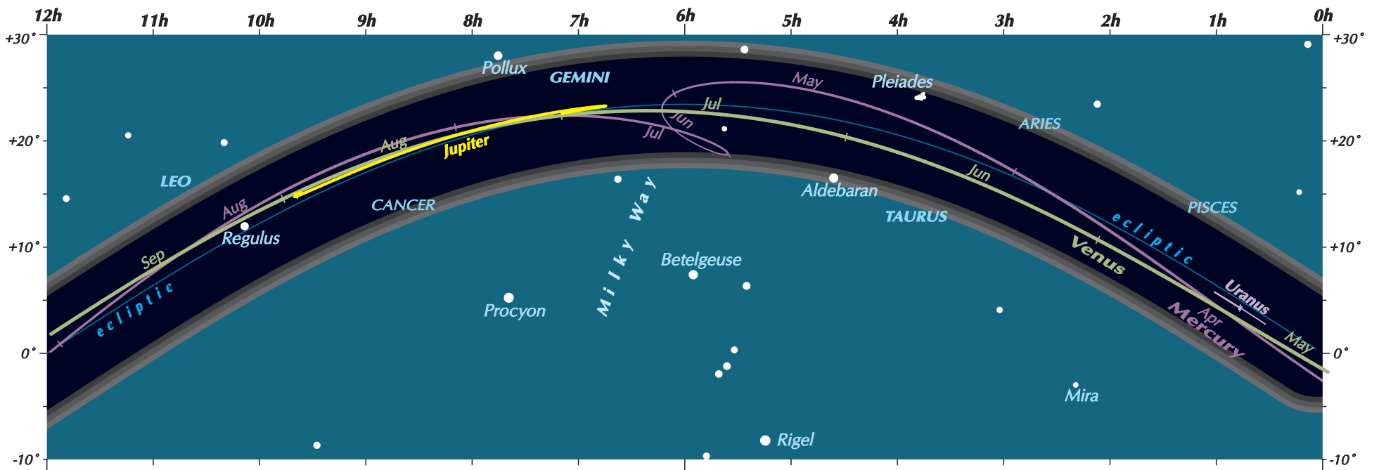
Maps of the planets' movements throughout the year. All but Pluto keep to the zodiacal band, not departing more than 8\frac{1}{2}^\circ from the ecliptic. Declination (vertical) scale is exaggerated by 1.5.
